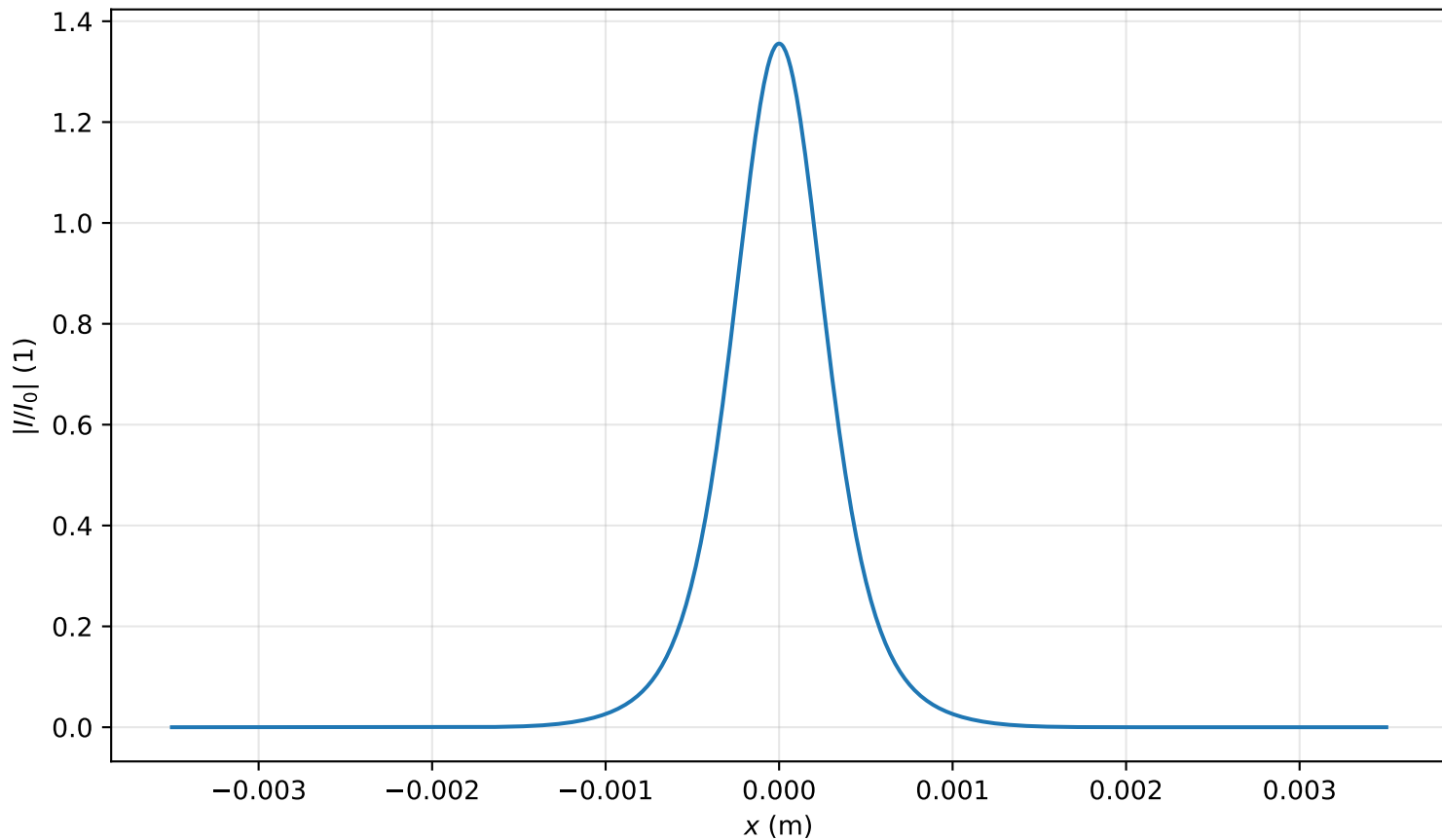
Intensity profile I(x, y = 0, z = 1.433m)/I_0 , P_{in}=0.8P_{cr} , artificial time
